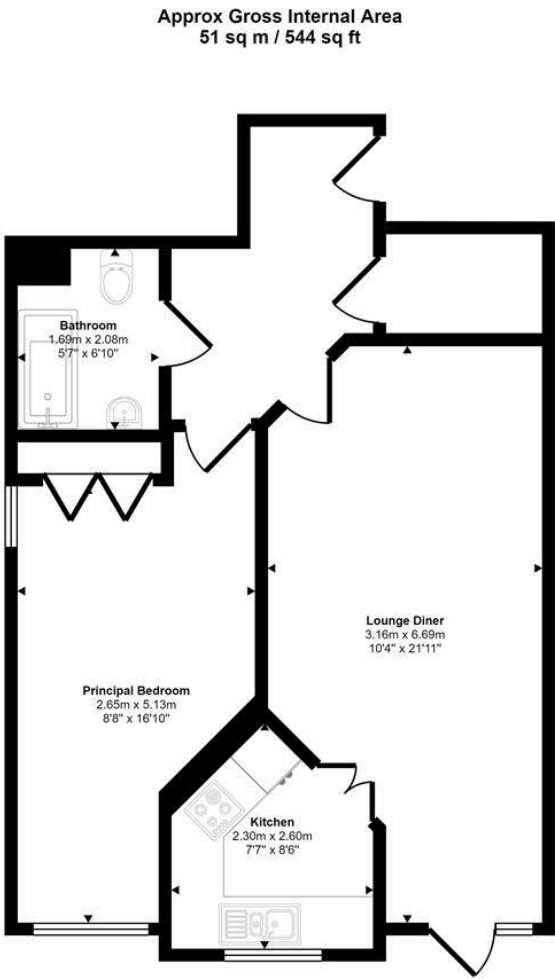
Floorplan
